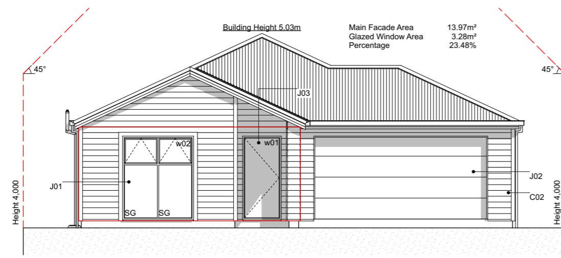
E-01 West Elevation Scale 1:100
